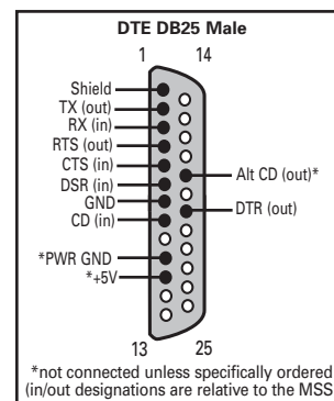
DB25 Serial Port Pinout (single) (Version B)
