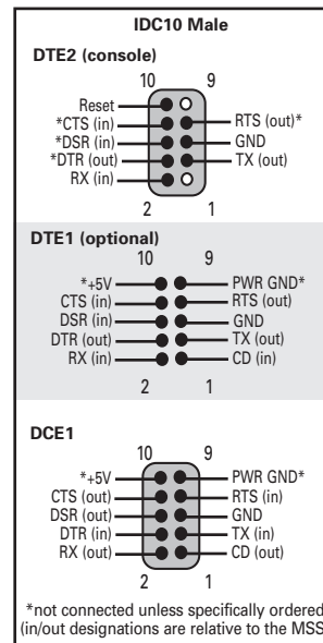
IDC10 Header Pinout (Version C)
