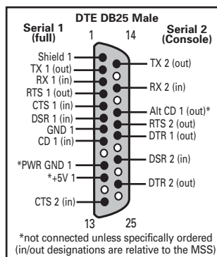
DB25 Serial Connector Pinout (double) (Version A)
